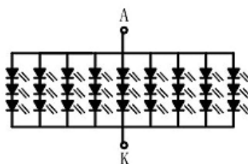
LED CIRCUIT DIAGRAM
