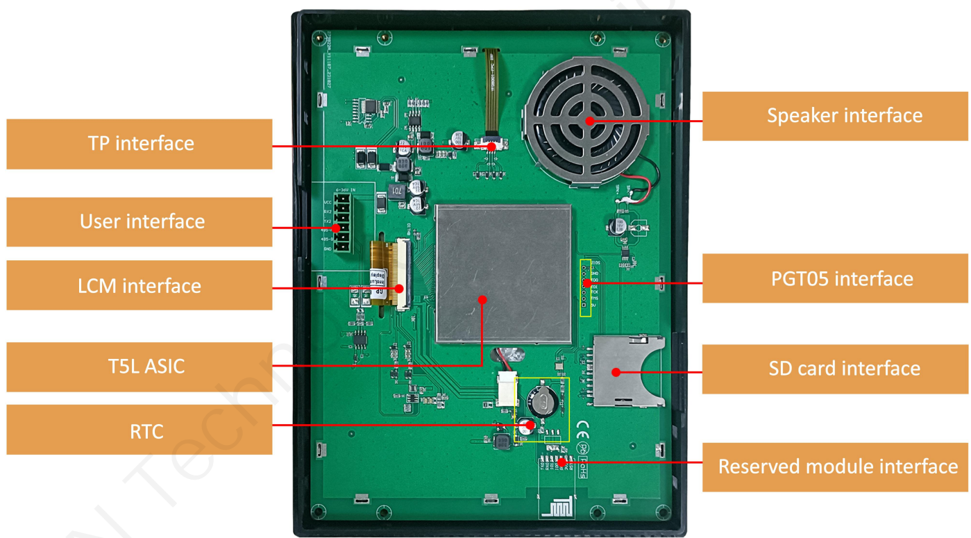
Hardware interface
